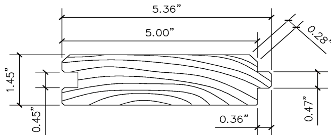
Section View of Typical Panel
